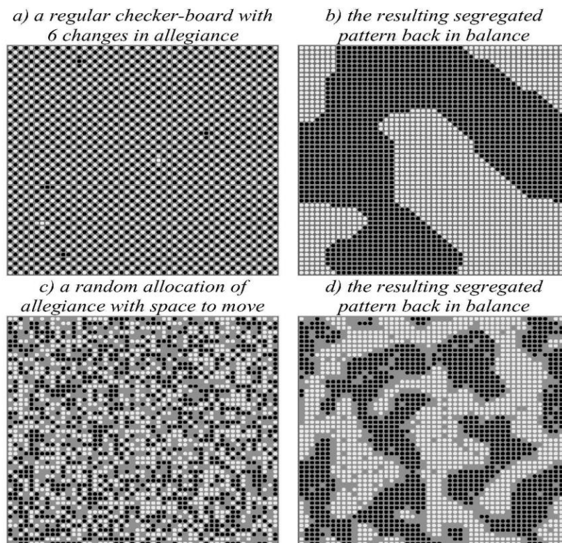
Figure 6: Emergent Segregation: A Fragile Equality (a) gives way to Segregation (b); A Random Mix (c) gives way to Segregation (d)
